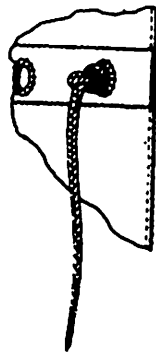
Full Size Practice (Braided Reef Point shown. Fasten with overhand knot. both sides of reef band hole.)
