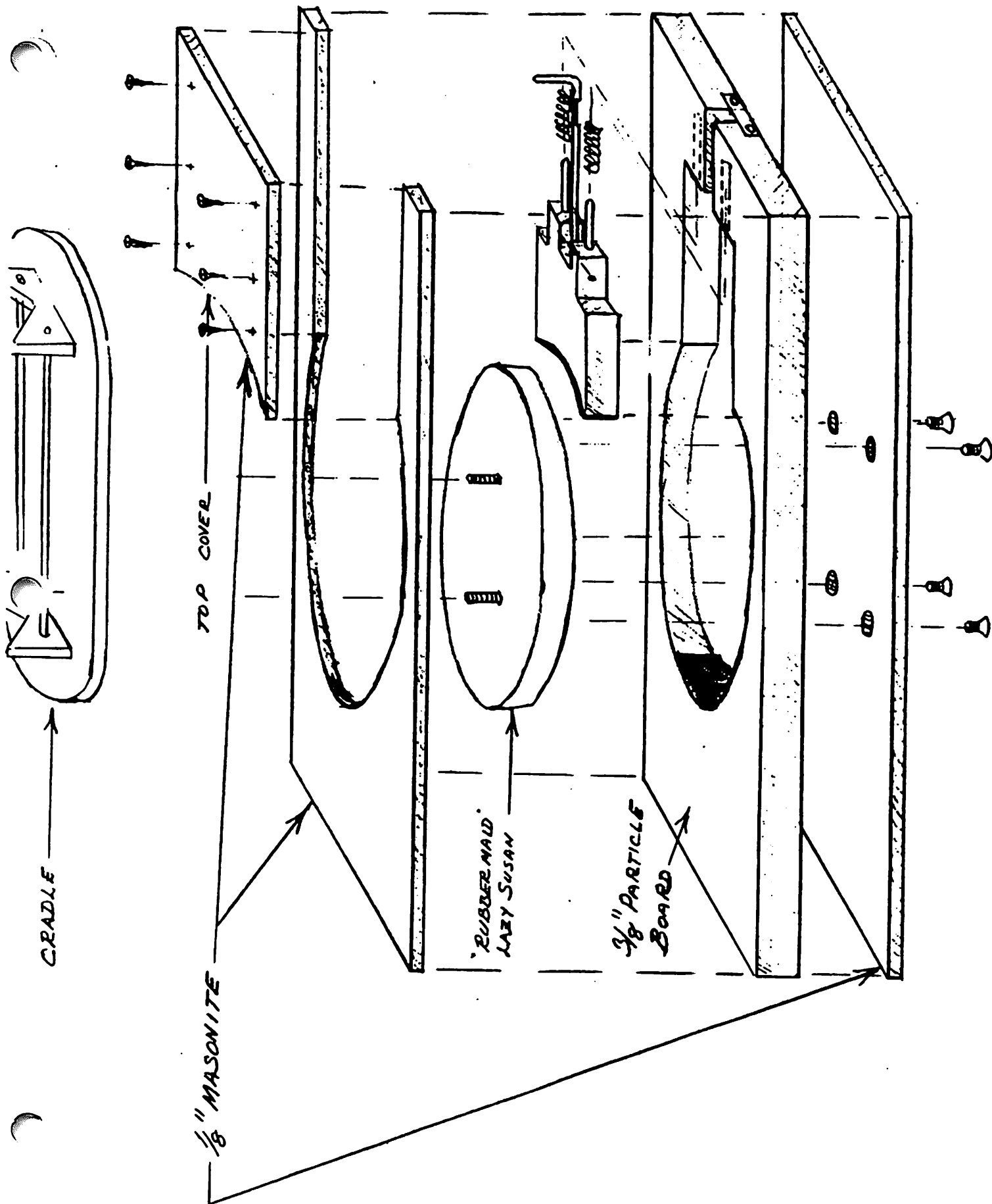
REVOLVING CRADLE ASSEMBLY DRAWING
